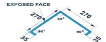
Corner Flashing
